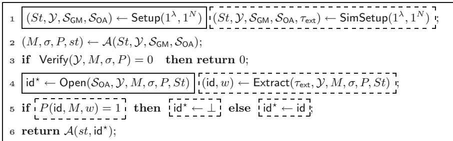
Fig. 2. Experiment \text{Exp}_{\mathcal{A}}^{\text{real}}(\lambda) (resp. \text{Exp}_{\mathcal{A}}^{\text{ext}}(\lambda) ) excluding the dotted (resp. solid) boxes.
