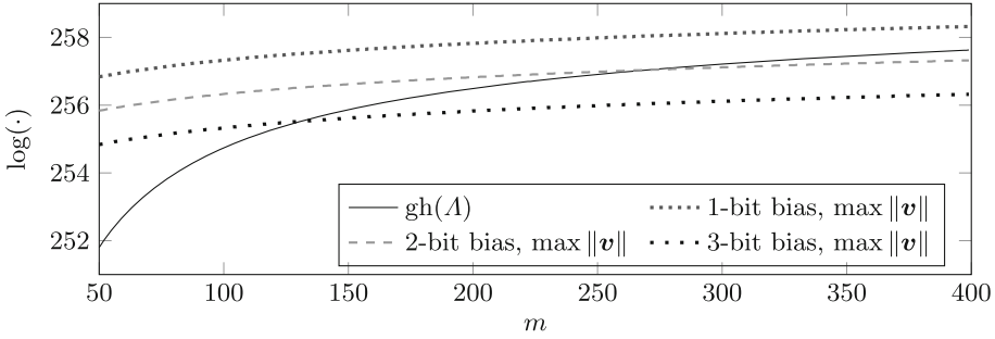
Fig. 2. Illustrating the “lattice barrier”. BDD is expected to become feasible when the length of the target vector \|\mathbf{v}\| is less than the Gaussian heuristic gh(\mathcal{A}) ; we plot the upper bound in Eq. (3) for \log(n) = 256 against varying number of samples m .
